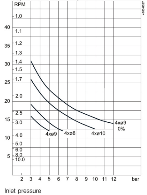
Cleaning Time, Complete Pattern Min. RPM of machine body PTM (Pattern time minutes)
